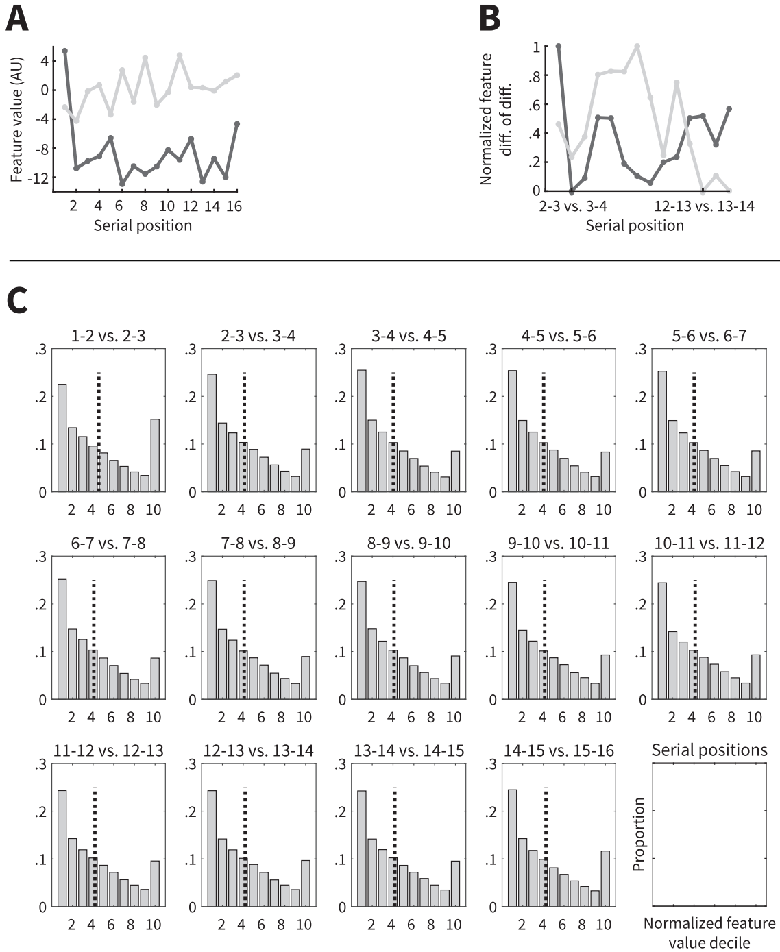
Figure B2 Histogram of Feature Value Differences Contributing to Each Feature Vector
