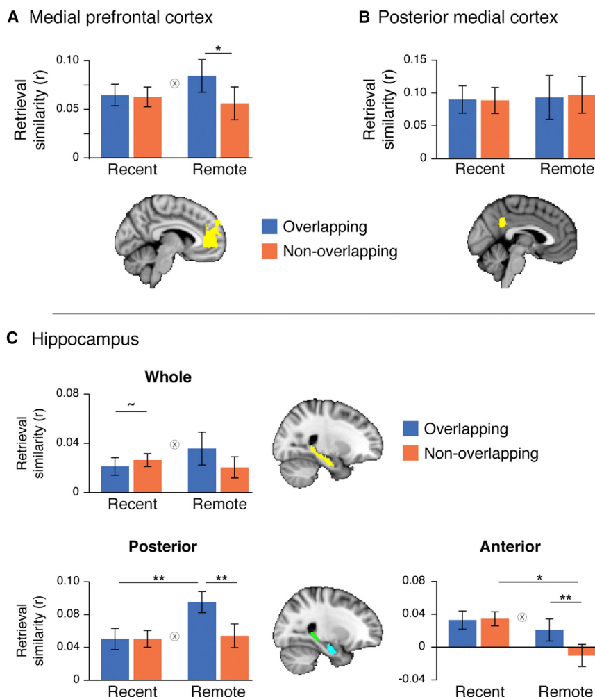
Figure 3. Retrieval Similarity
