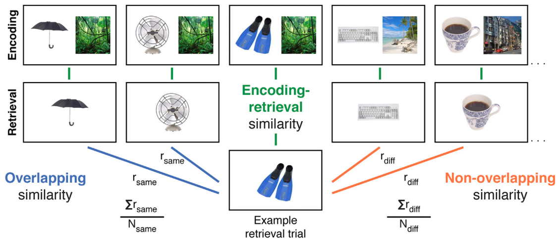
Figure 2. Analysis Approach
