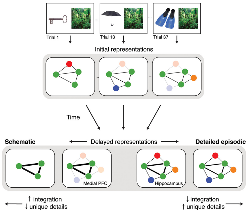
Figure 6. Schematic of the Theorized Neural Transformation of Overlapping Episodic Memories
